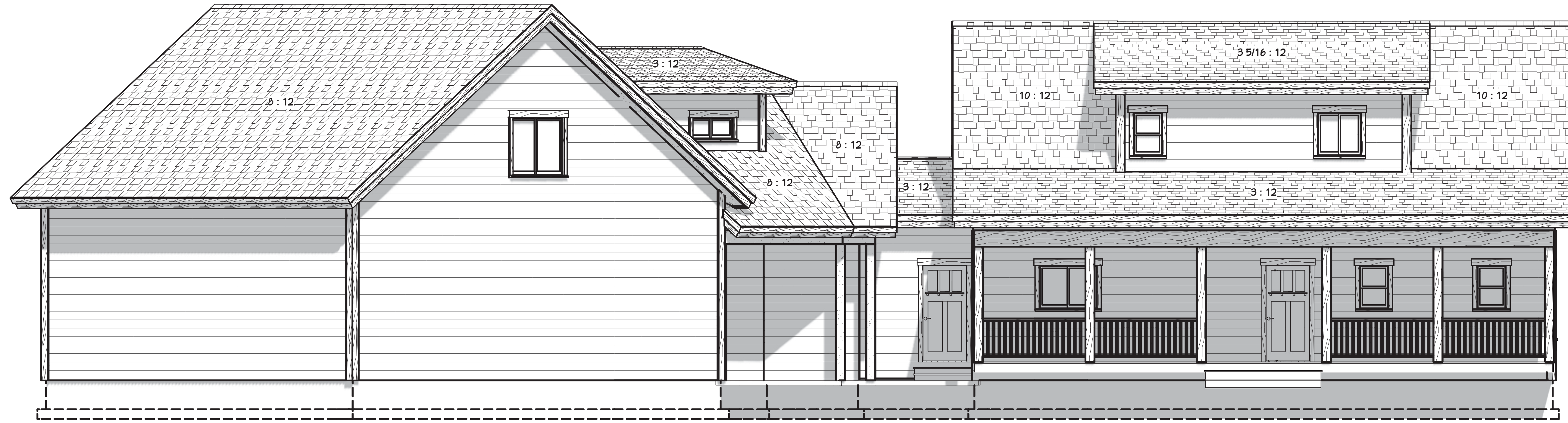
REAR ELEVATION 1/4" = 1'-0"
