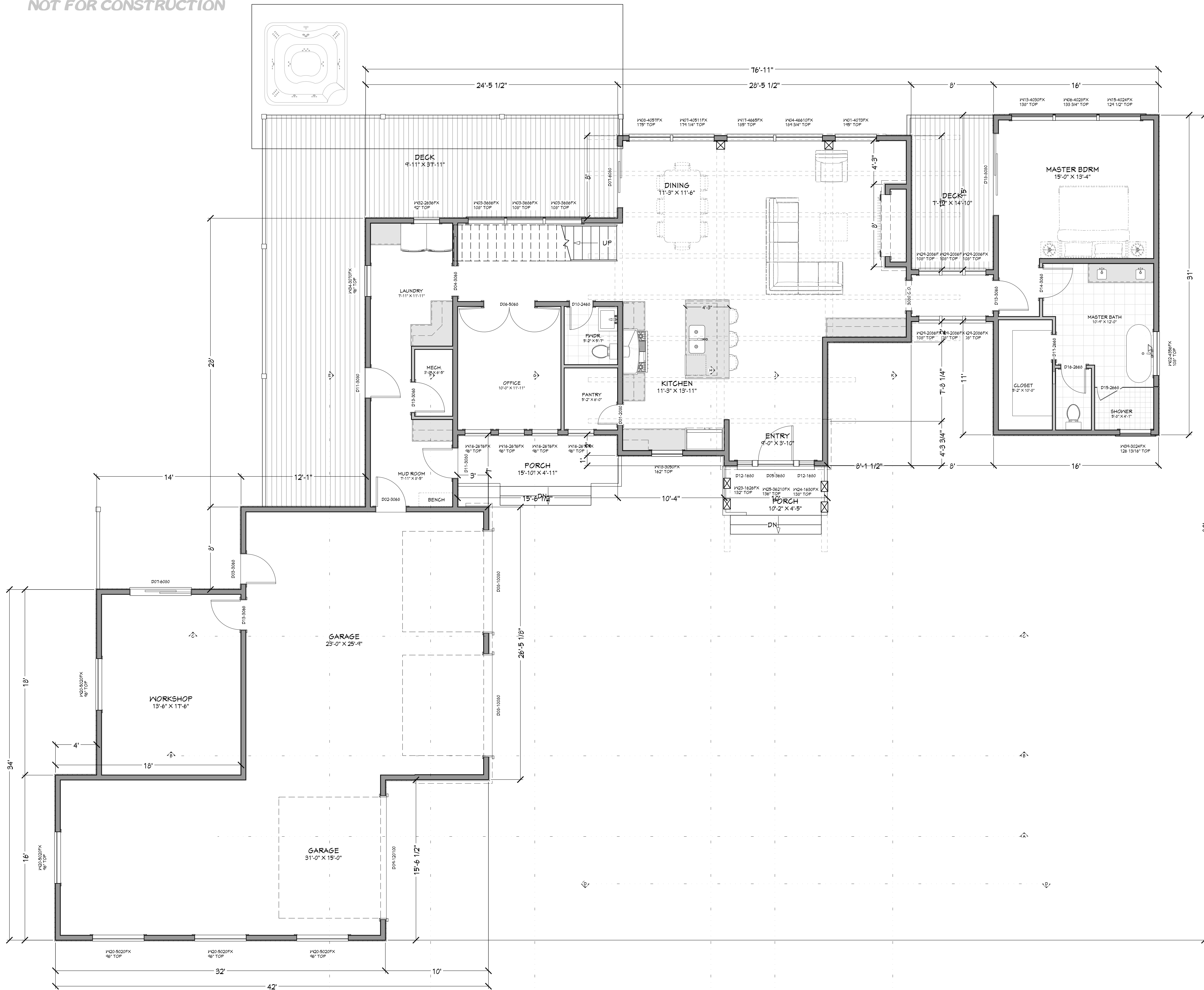
FLOOR PLAN - 1ST LEVEL 1/4 IN = 1 FT
