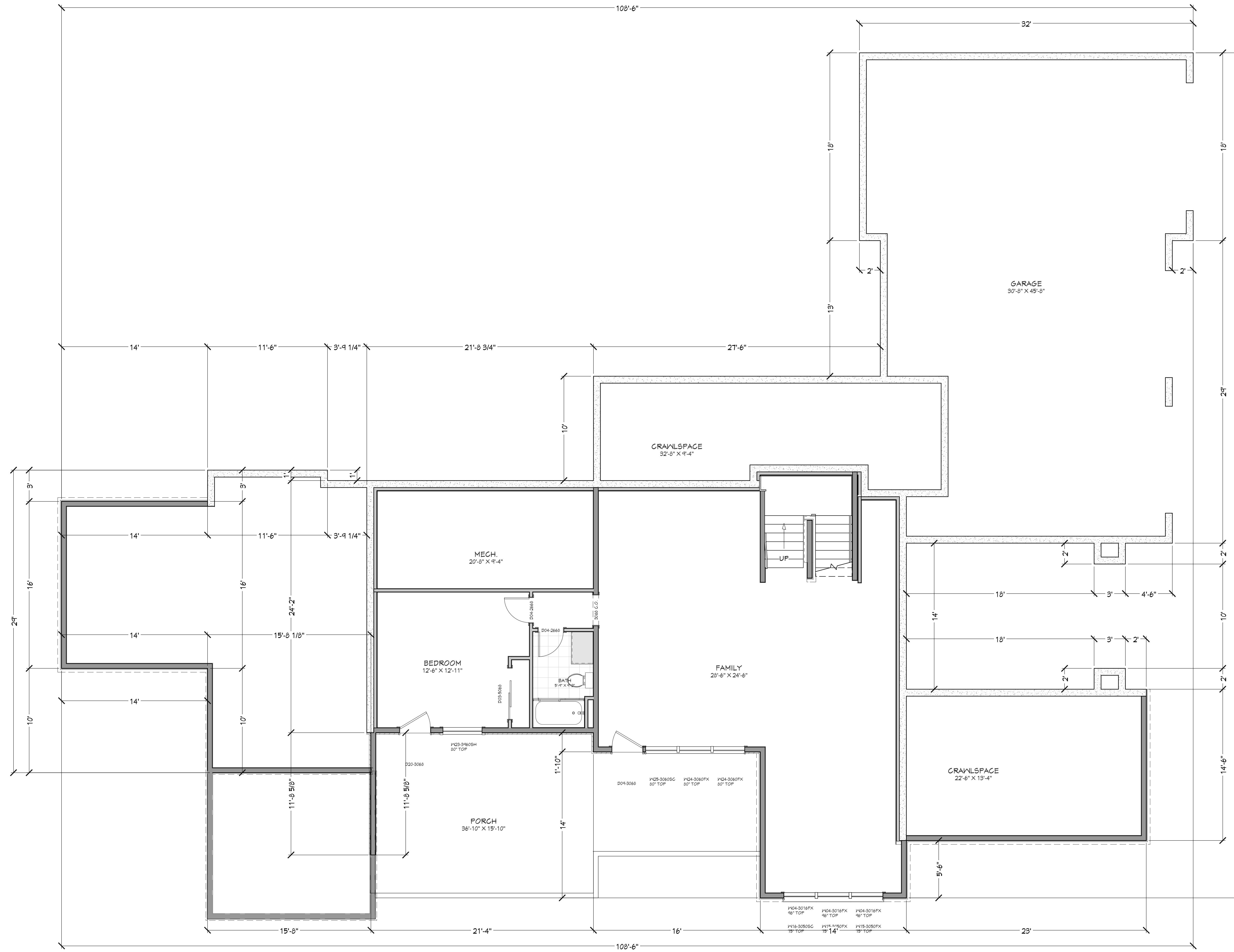
FLOOR PLAN - BASEMENT 1/4 IN = 1 FT
