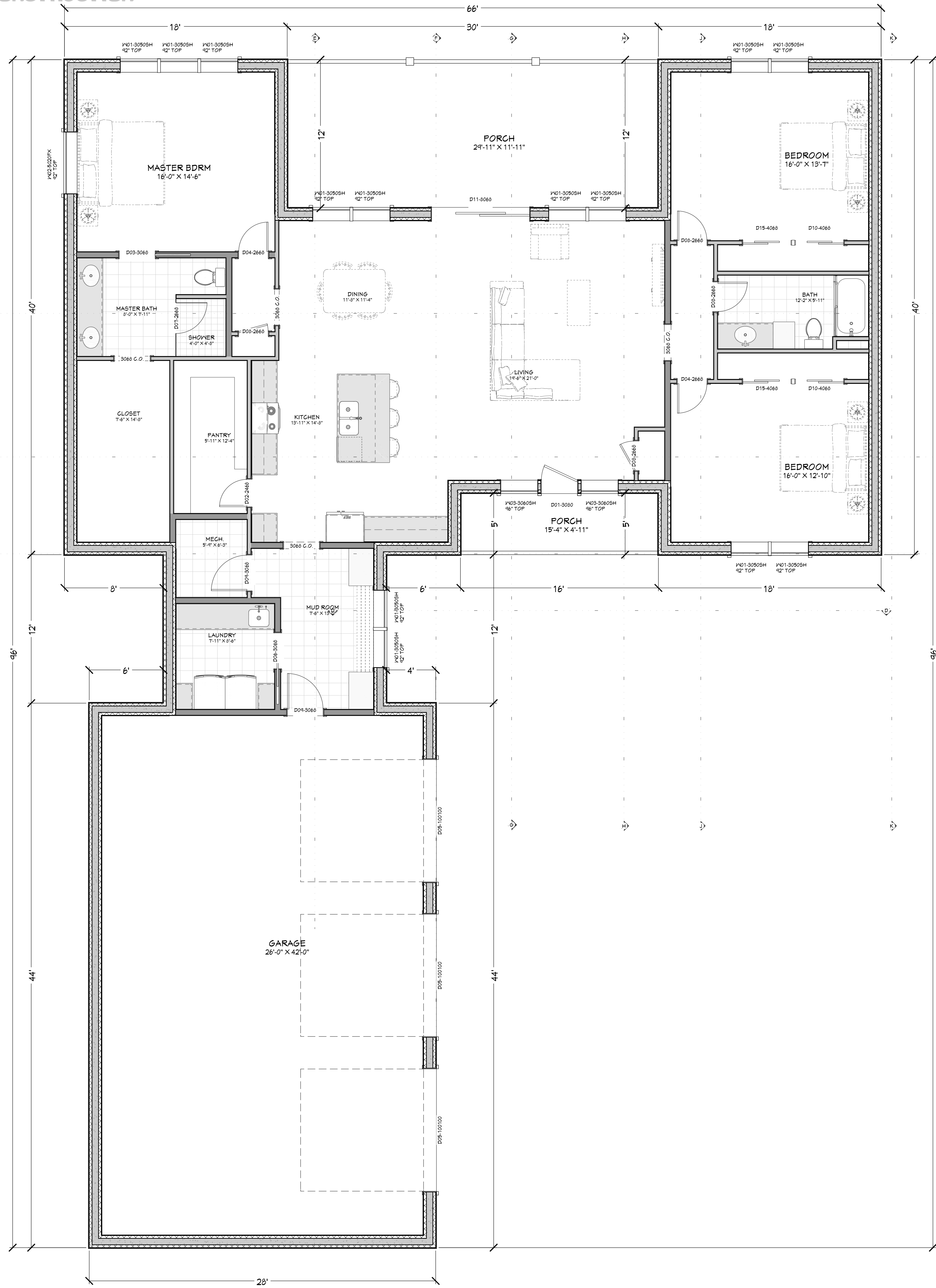
FLOOR PLAN - 1ST LEVEL 1/4 IN = 1 FT
