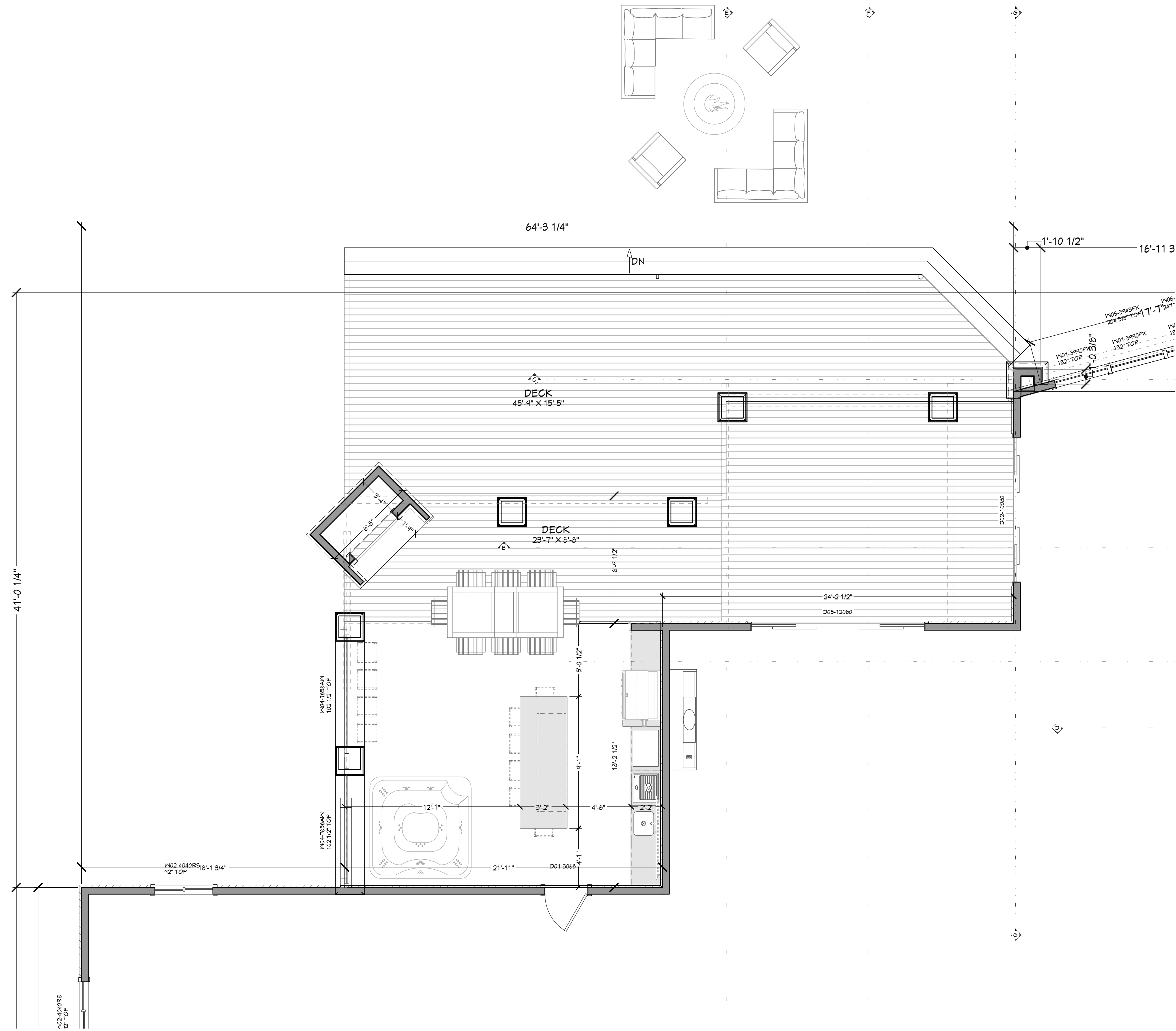
FLOOR PLAN - 1ST LEVEL 1/4" = 1'-0"
