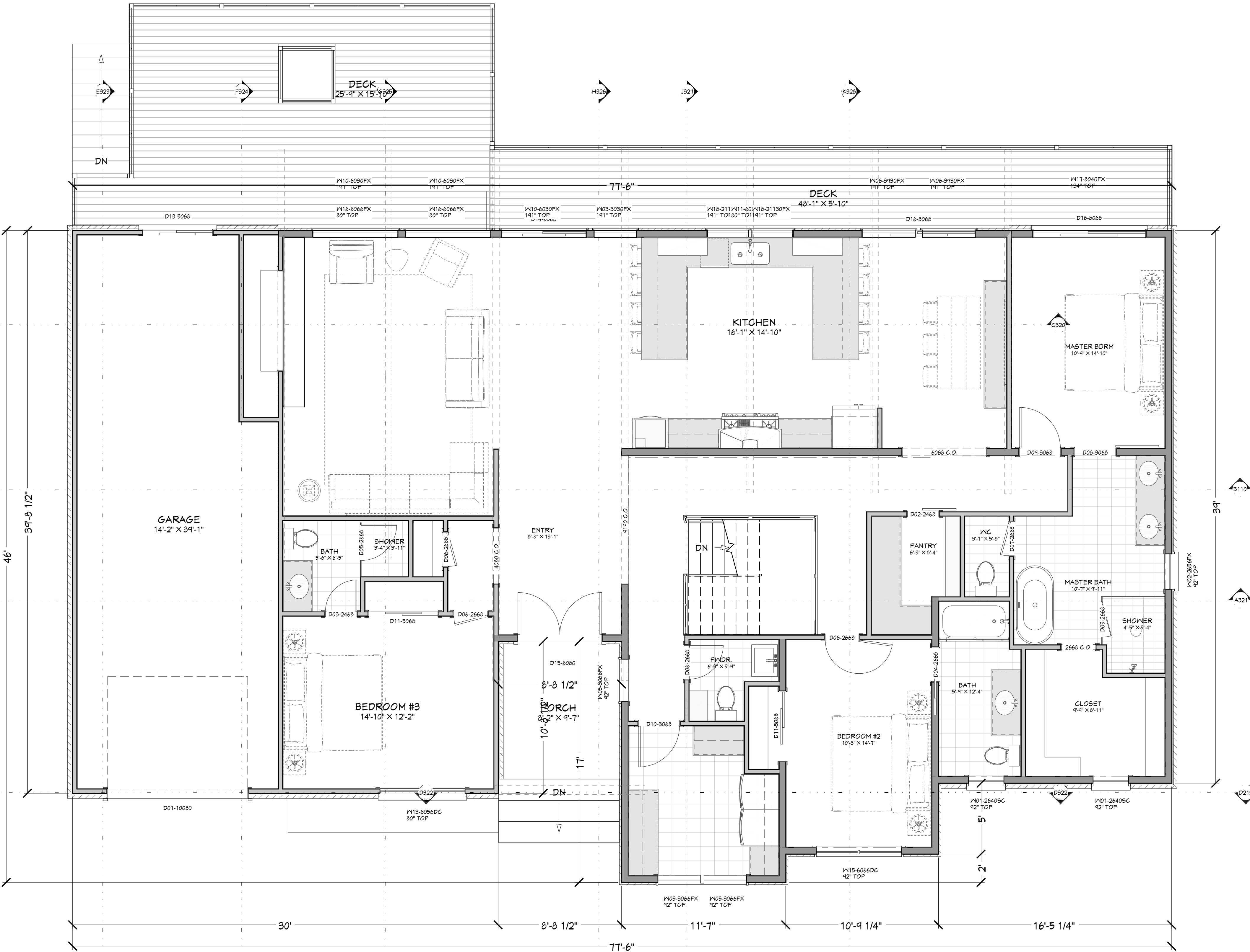
FLOOR PLAN - 1ST LEVEL 1/4 IN = 1 FT
