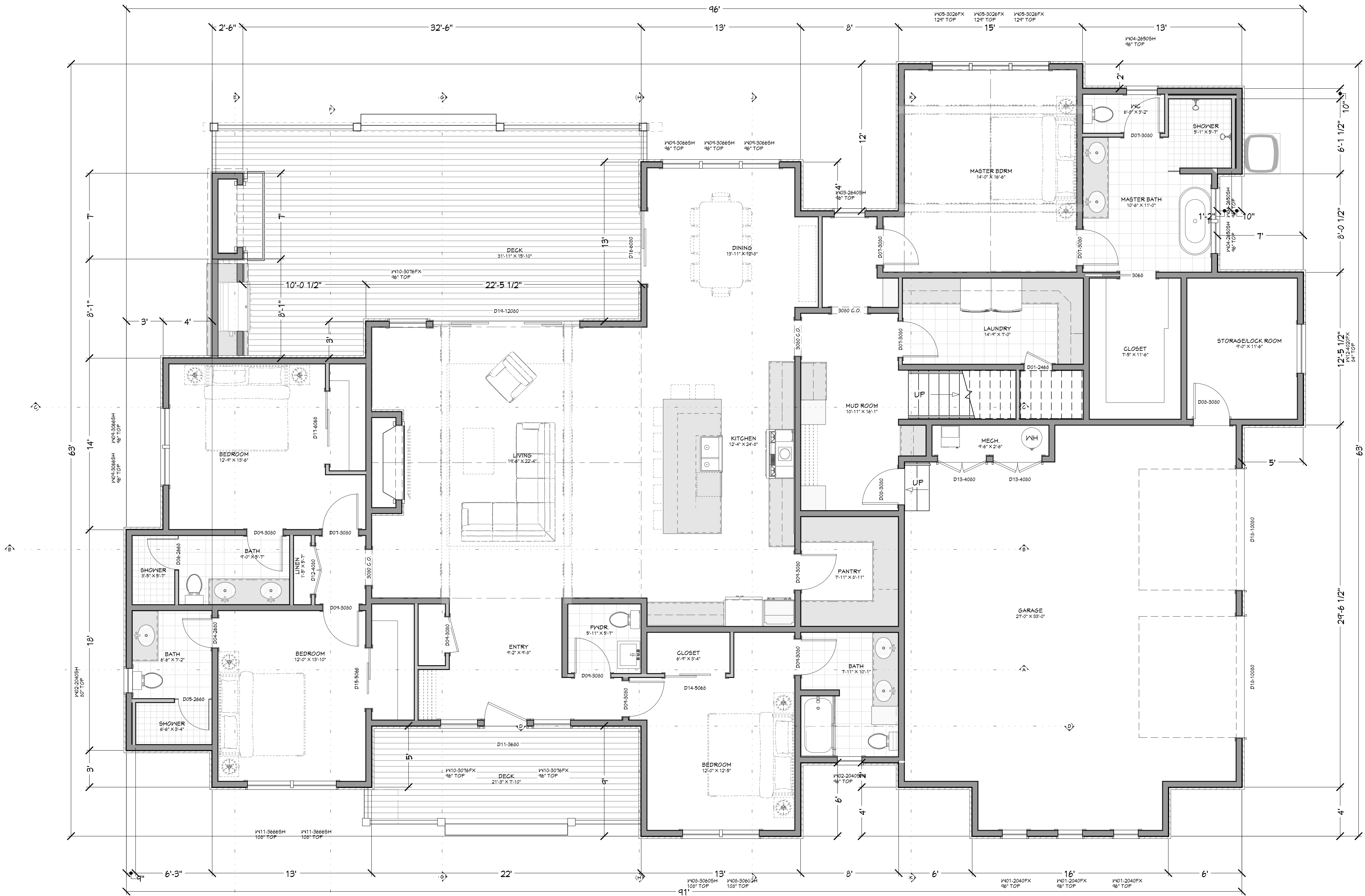
FLOOR PLAN - 1ST LEVEL 1/4 IN = 1 FT
